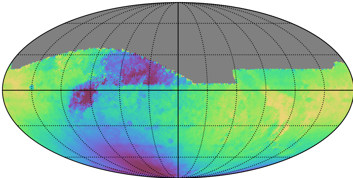
weather_cloudso30v3.4_10yrs All sky r band: Median solarElong
