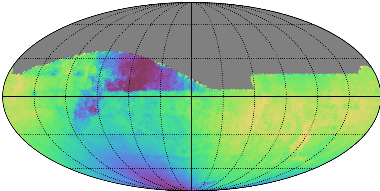
weather_cloudso30v3.4_10yrs All sky i band: Median solarElong
