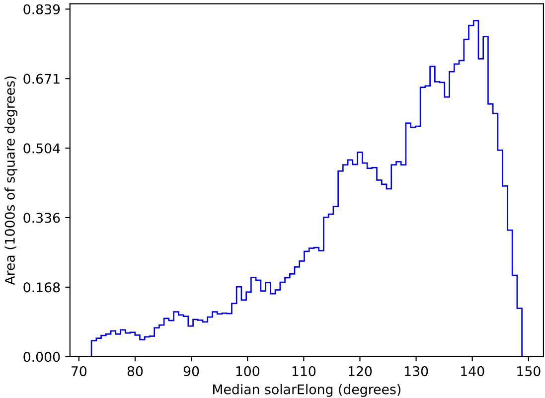
weather_cloudso30v3.4_10yrs All sky i band: Median solarElong
