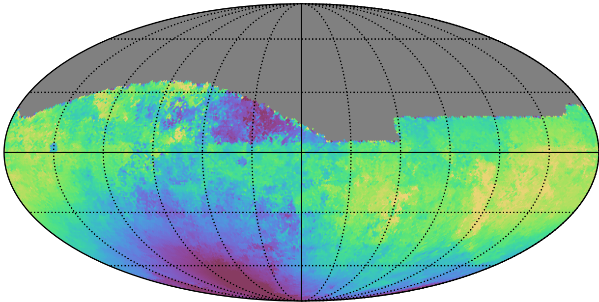
weather_cloudso30v3.4_10yrs All sky g band: Median solarElong
