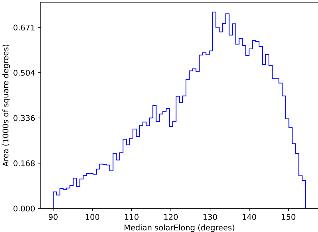
weather_cloudso30v3.4_10yrs All sky g band: Median solarElong
