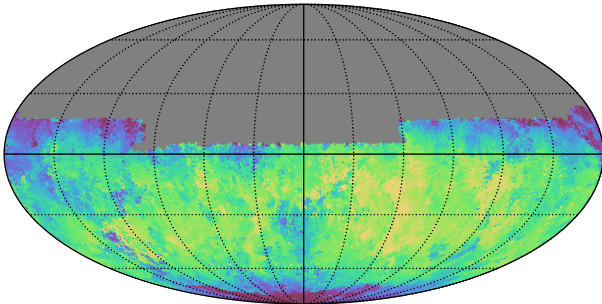
weather_cloudso30v3.4_10yrs Yr 1 y band: Median skyBrightness
