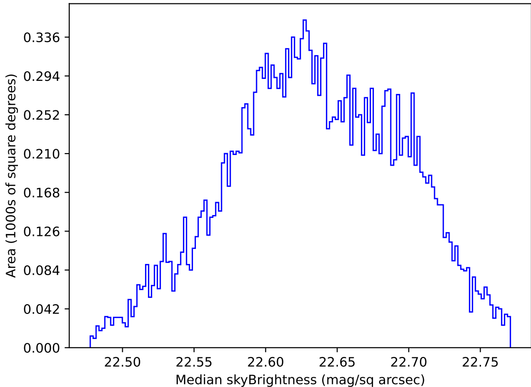
weather_cloudso30v3.4_10yrs Yr 1 u band: Median skyBrightness
