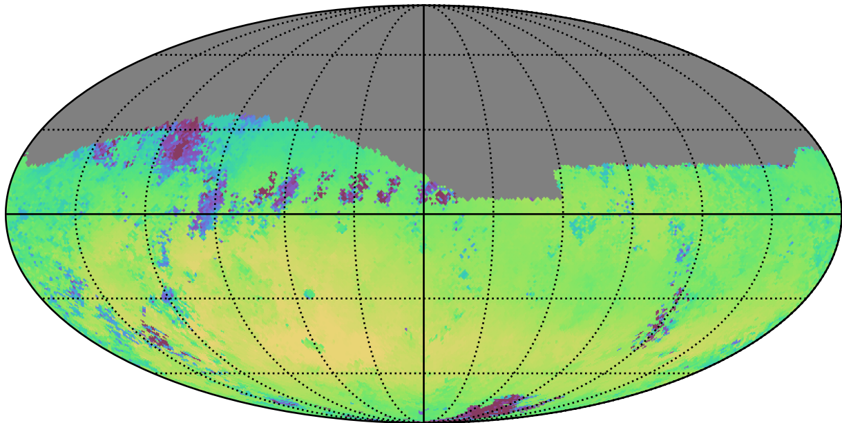
weather_cloudso30v3.4_10yrs Yr 1 r band: Median skyBrightness
