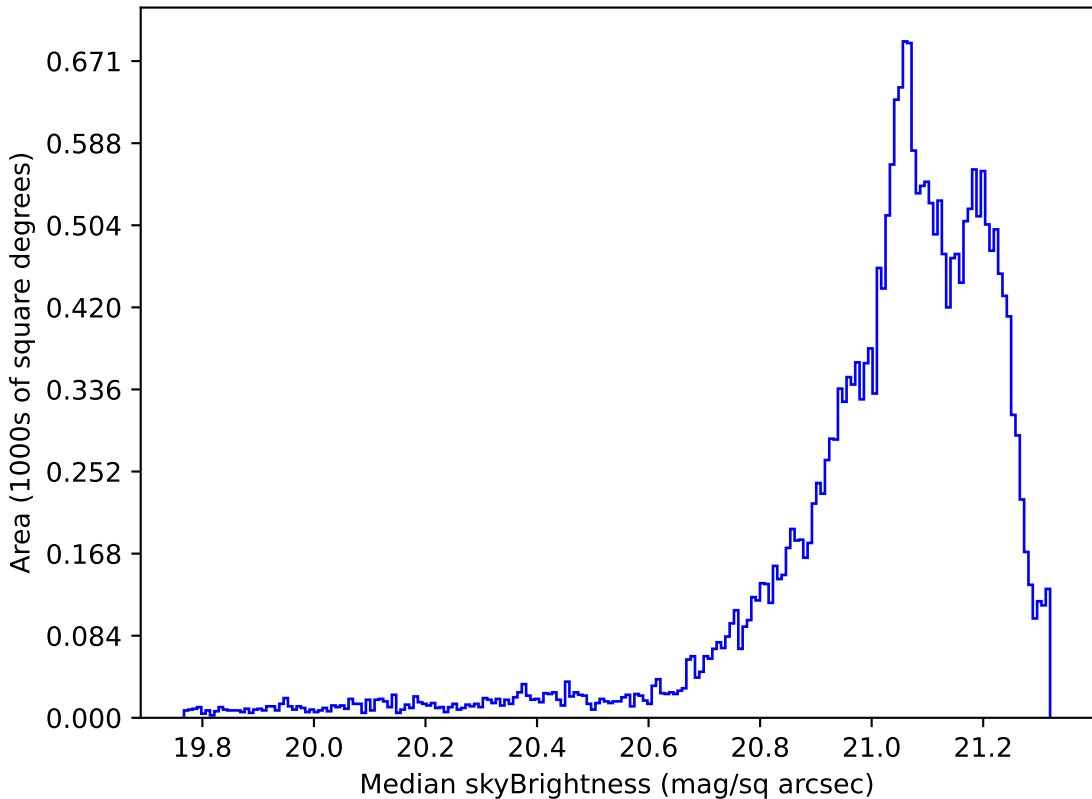
weather_cloudso30v3.4_10yrs Yr 1 r band: Median skyBrightness
