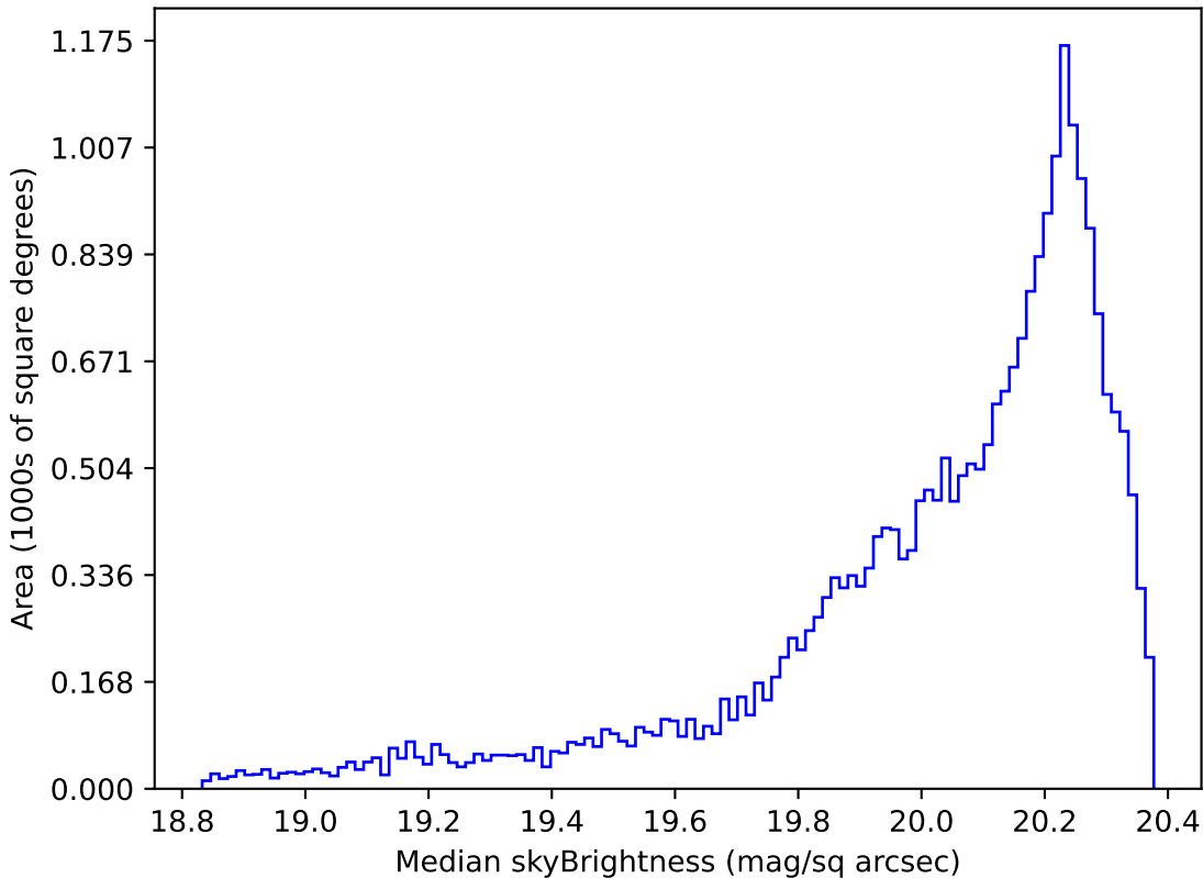
weather_cloudso30v3.4_10yrs Yr 1 i band: Median skyBrightness
