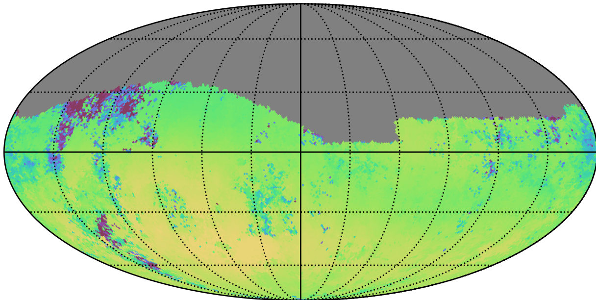
weather_cloudso30v3.4_10yrs Yr 1 g band: Median skyBrightness
