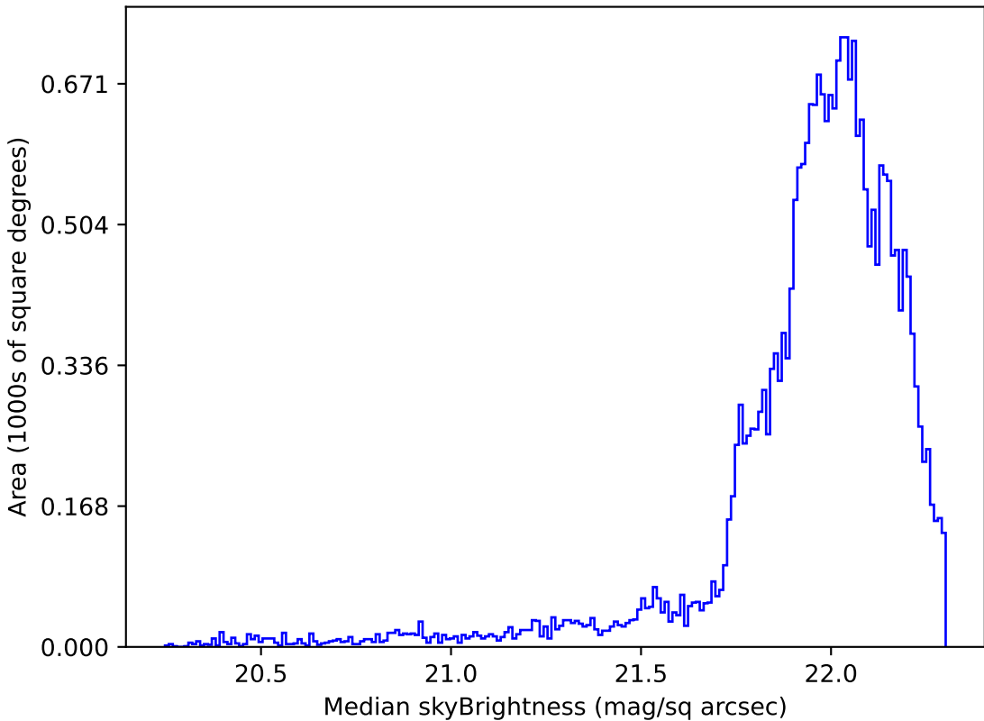
weather_cloudso30v3.4_10yrs Yr 1 g band: Median skyBrightness
