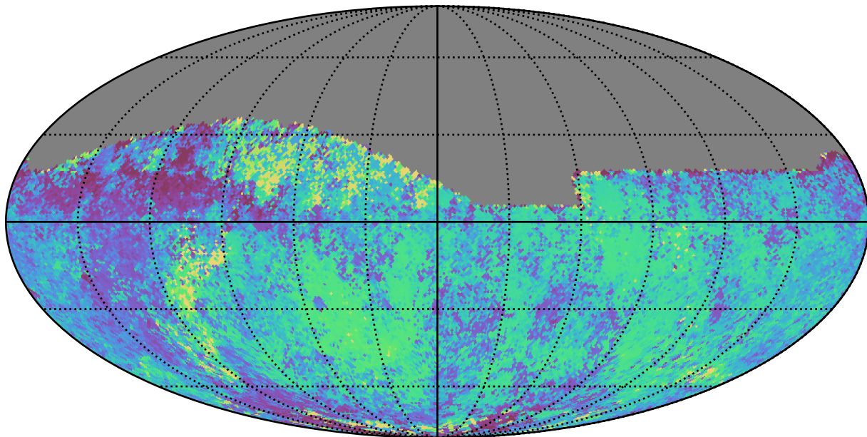
weather_cloudso30v3.4_10yrs Yr 1 all bands: Median skyBrightness
