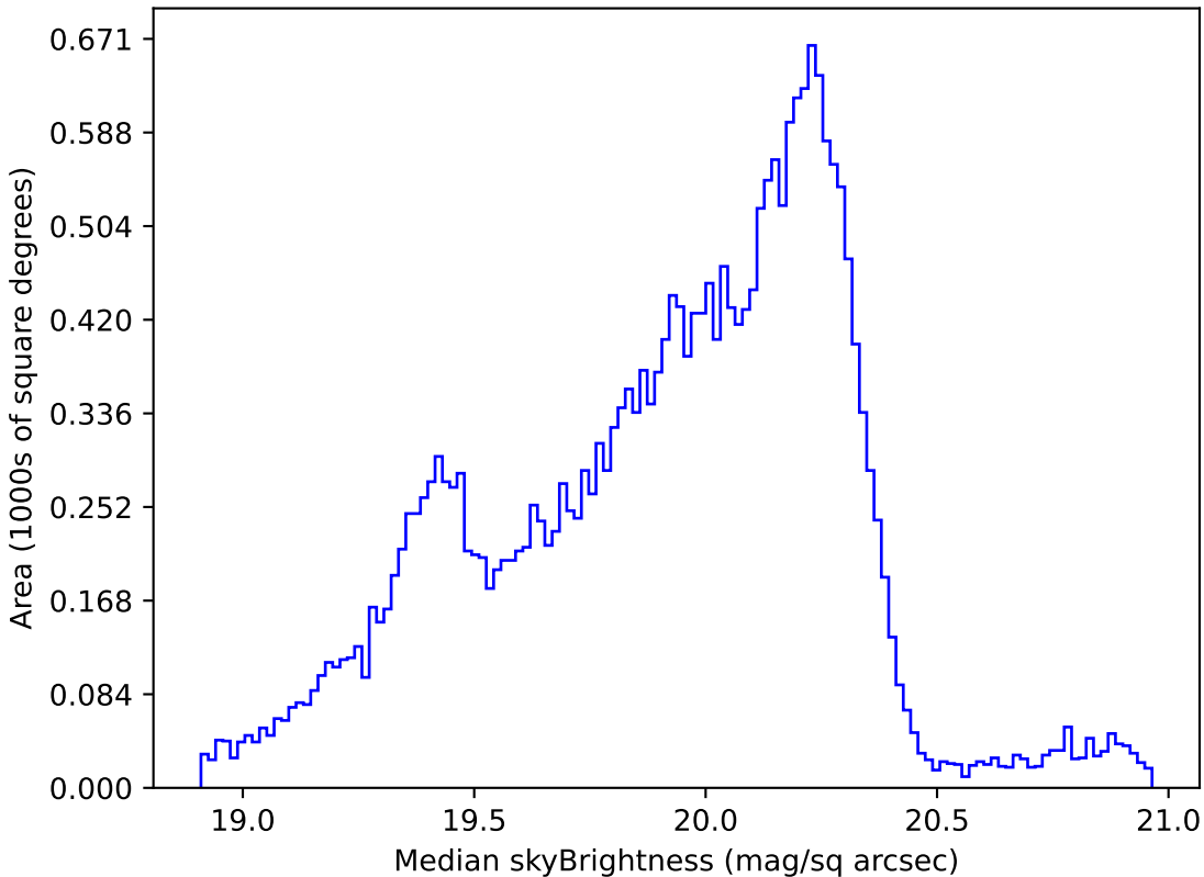
weather_cloudso30v3.4_10yrs Yr 1 all bands: Median skyBrightness
