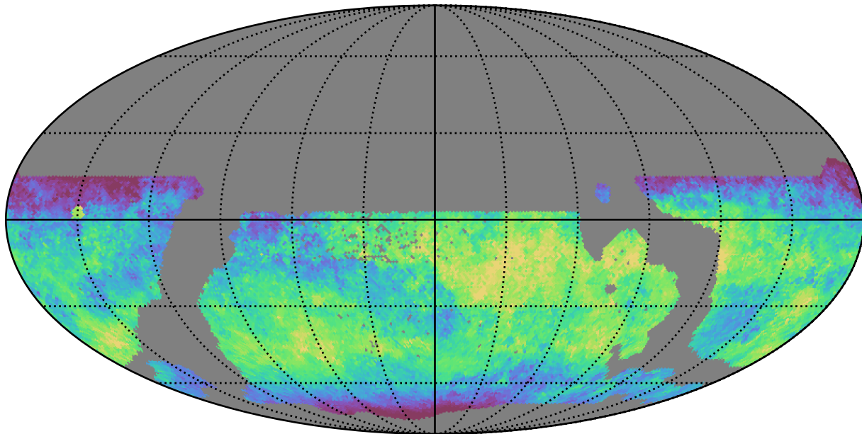
weather_cloudso30v3.4_10yrs WFD z band: Median skyBrightness
