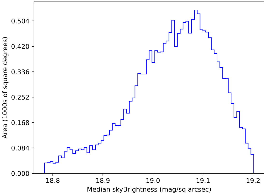
weather_cloudso30v3.4_10yrs WFD z band: Median skyBrightness
