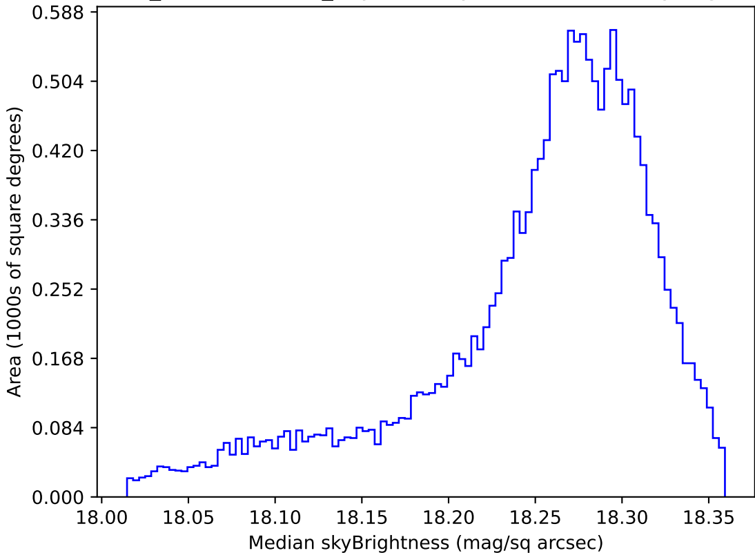
weather_cloudso30v3.4_10yrs WFD y band: Median skyBrightness
