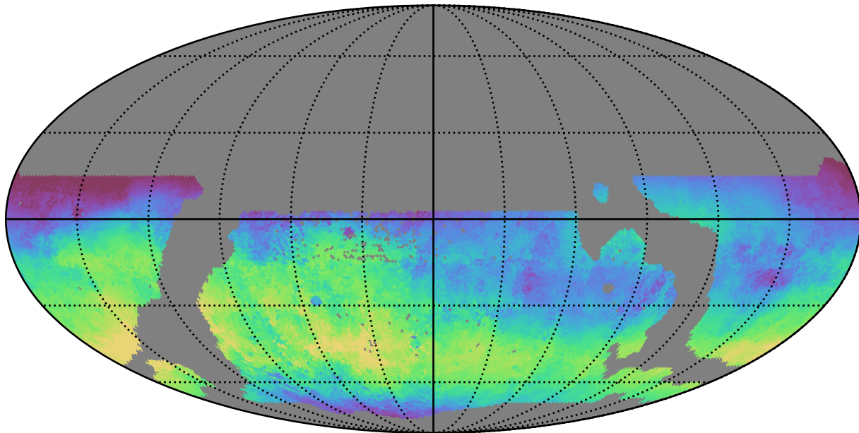
weather_cloudso30v3.4_10yrs WFD u band: Median skyBrightness
