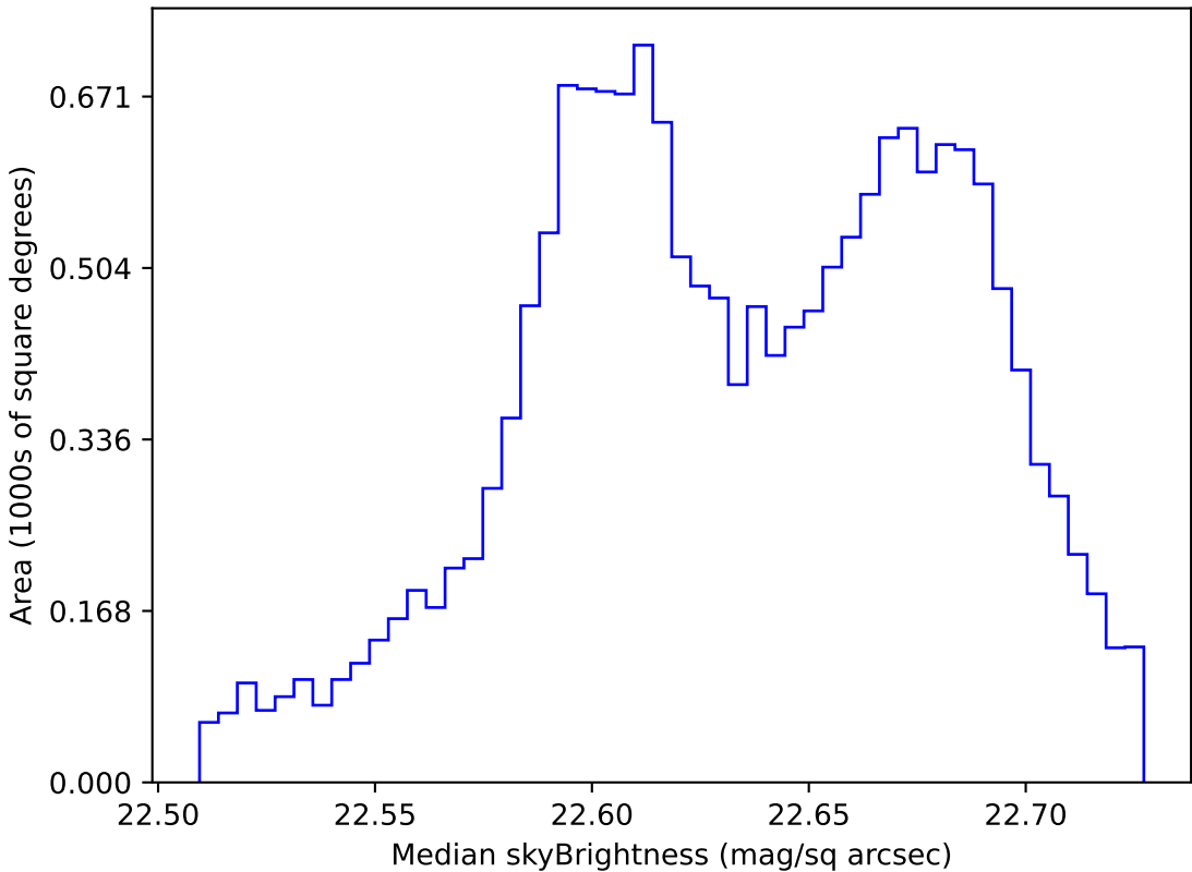
weather_cloudso30v3.4_10yrs WFD u band: Median skyBrightness
