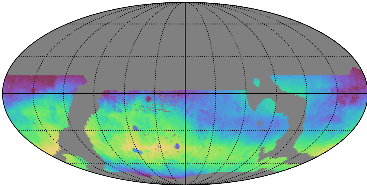
weather_cloudso30v3.4_10yrs WFD r band: Median skyBrightness
