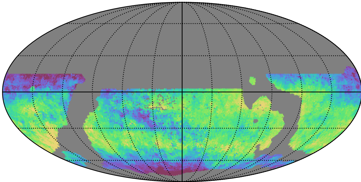
weather_cloudso30v3.4_10yrs WFD i band: Median skyBrightness
