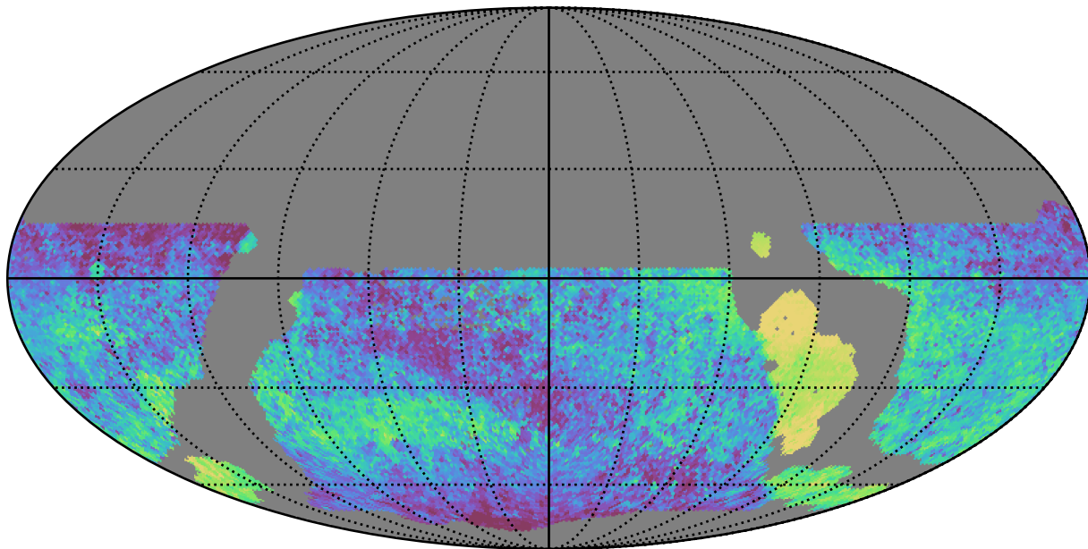
weather_cloudso30v3.4_10yrs WFD all bands: Median skyBrightness
