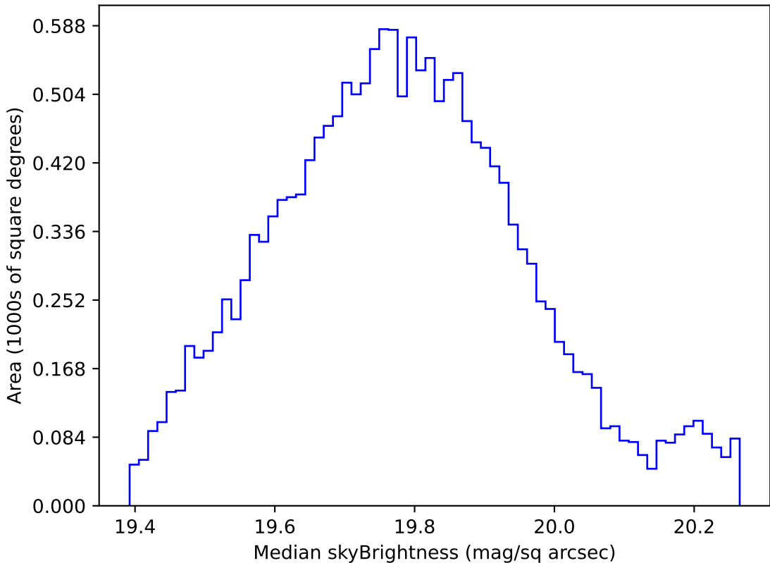
weather_cloudso30v3.4_10yrs WFD all bands: Median skyBrightness
