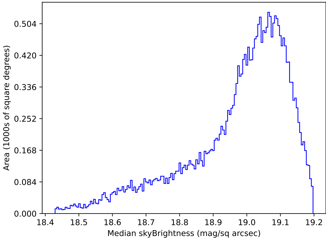
weather_cloudso30v3.4_10yrs All sky z band: Median skyBrightness
