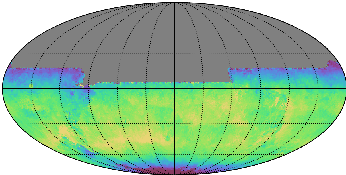
weather_cloudso30v3.4_10yrs All sky y band: Median skyBrightness
