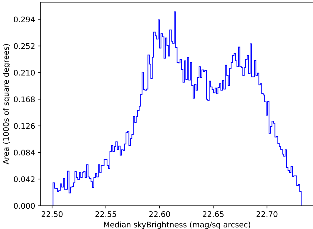
weather_cloudso30v3.4_10yrs All sky u band: Median skyBrightness
