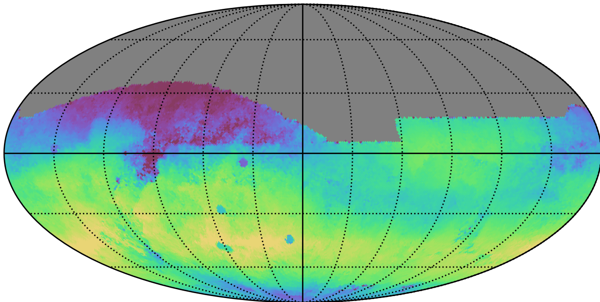
weather_cloudso30v3.4_10yrs All sky r band: Median skyBrightness
