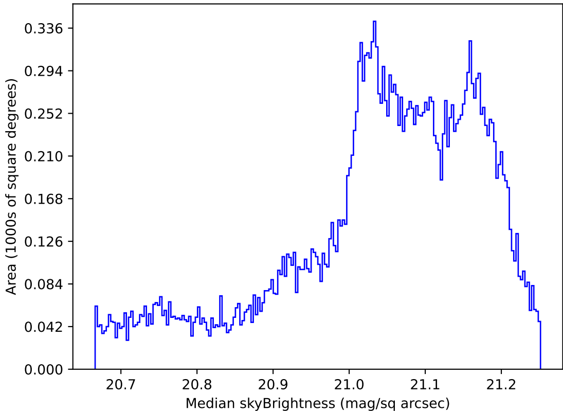
weather_cloudso30v3.4_10yrs All sky r band: Median skyBrightness
