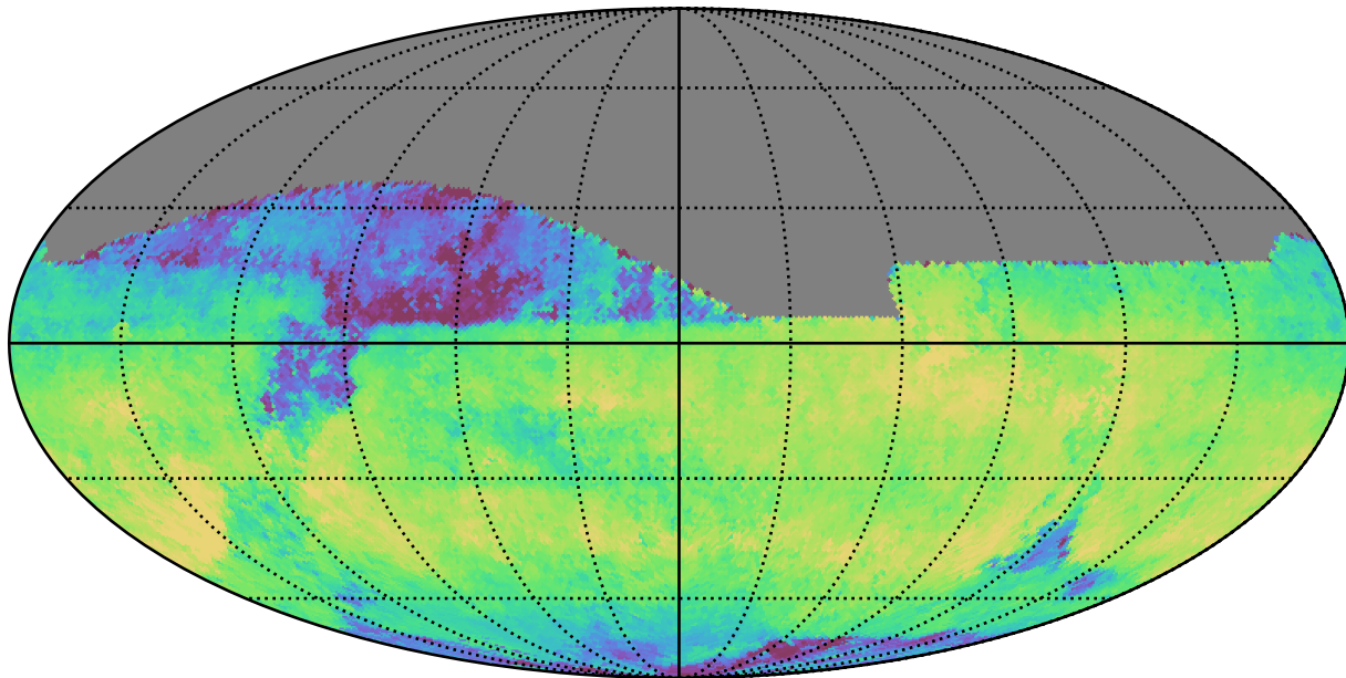
weather_cloudso30v3.4_10yrs All sky i band: Median skyBrightness
