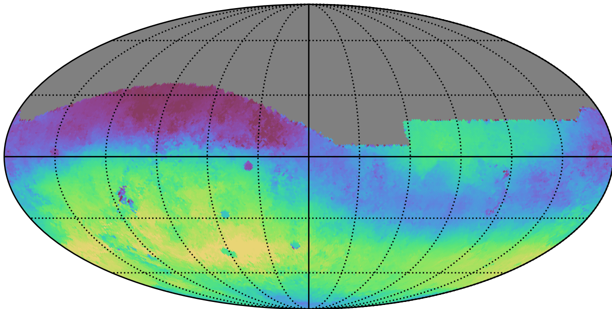
weather_cloudso30v3.4_10yrs All sky g band: Median skyBrightness
