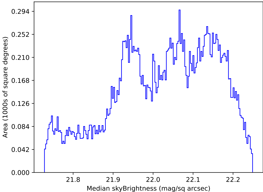
weather_cloudso30v3.4_10yrs All sky g band: Median skyBrightness
