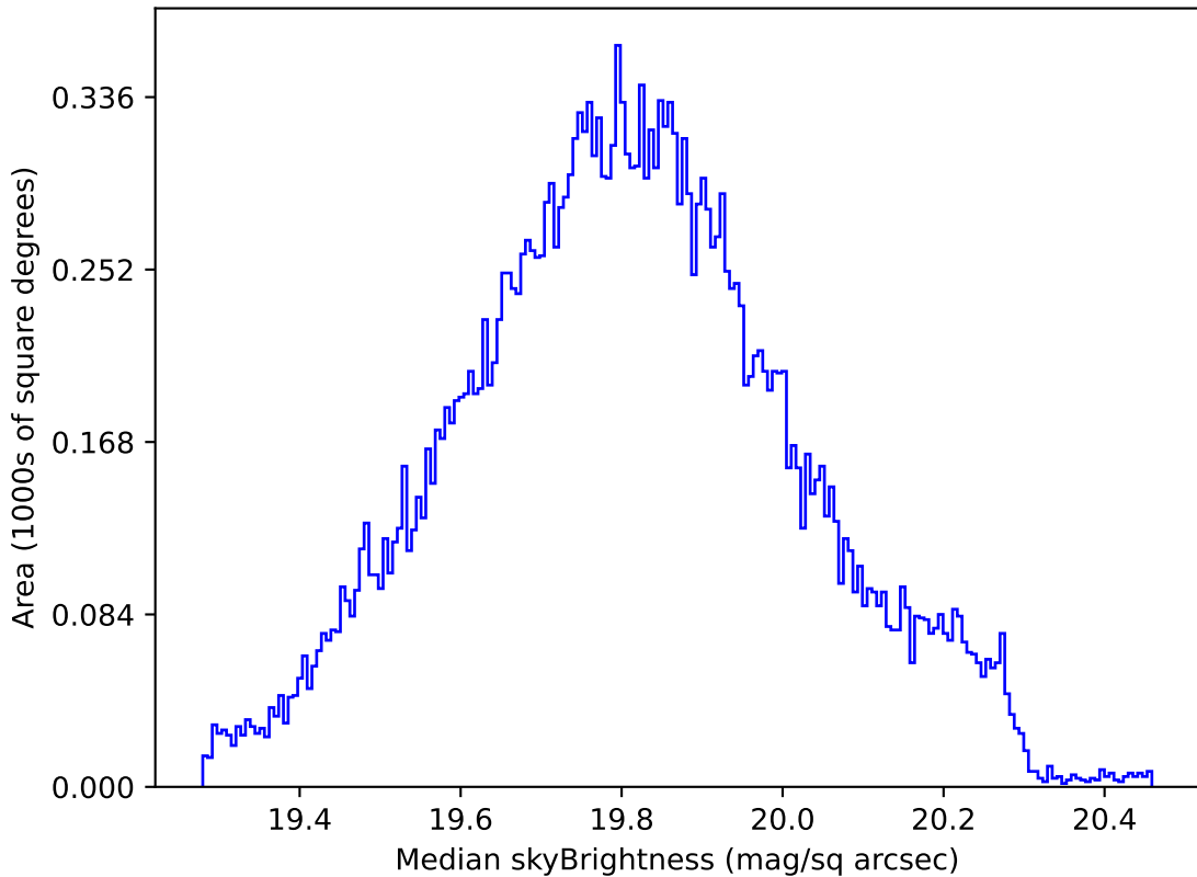
weather_cloudso30v3.4_10yrs All sky all bands: Median skyBrightness
