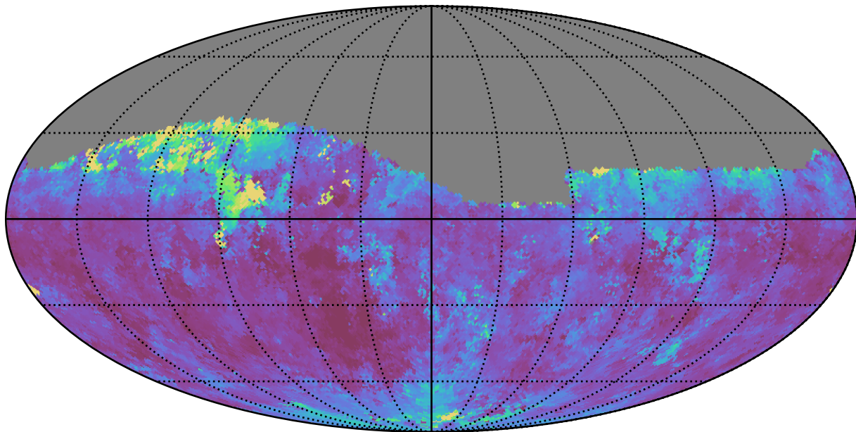
weather_cloudso30v3.4_10yrs Yr 1 z band: Median seeingGeom
