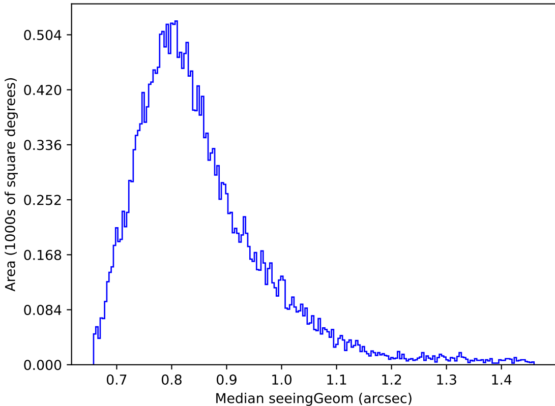
weather_cloudso30v3.4_10yrs Yr 1 z band: Median seeingGeom
