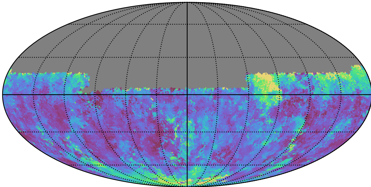
weather_cloudso30v3.4_10yrs Yr 1 y band: Median seeingGeom
