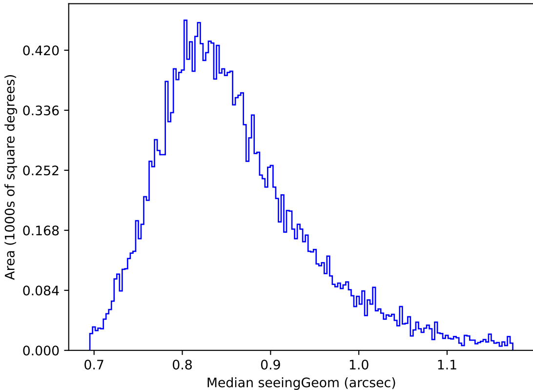
weather_cloudso30v3.4_10yrs Yr 1 y band: Median seeingGeom
