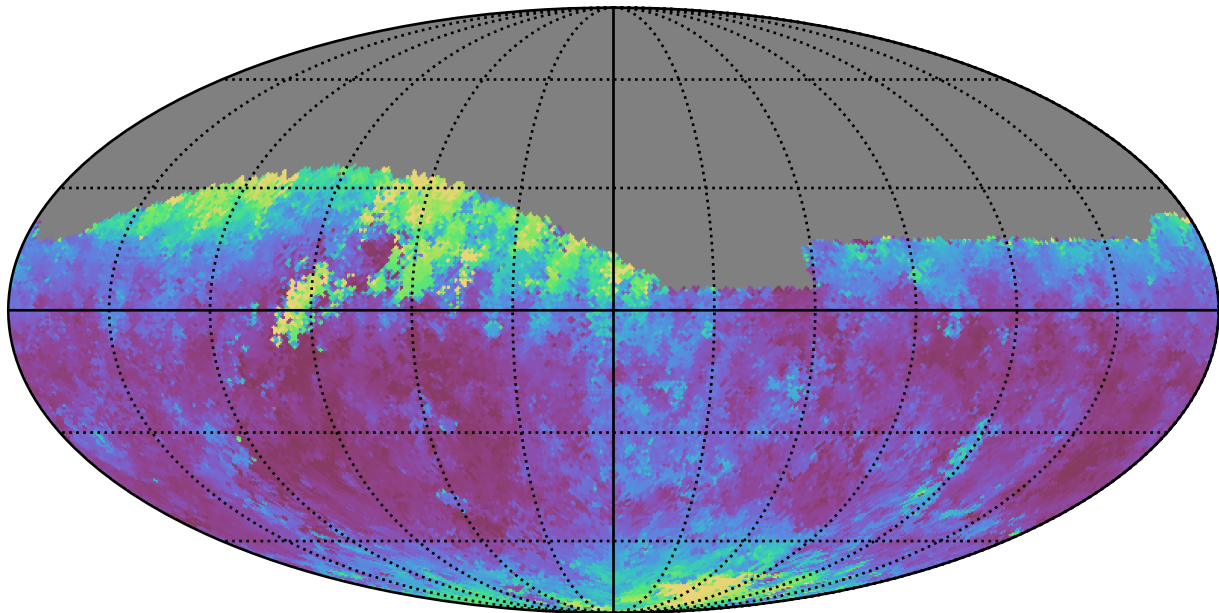
weather_cloudso30v3.4_10yrs Yr 1 r band: Median seeingGeom
