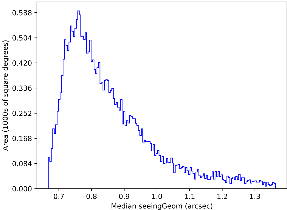
weather_cloudso30v3.4_10yrs Yr 1 r band: Median seeingGeom
