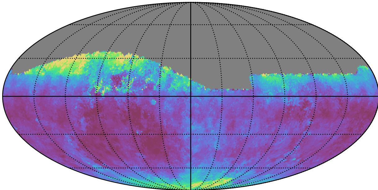
weather_cloudso30v3.4_10yrs Yr 1 all bands: Median seeingGeom
