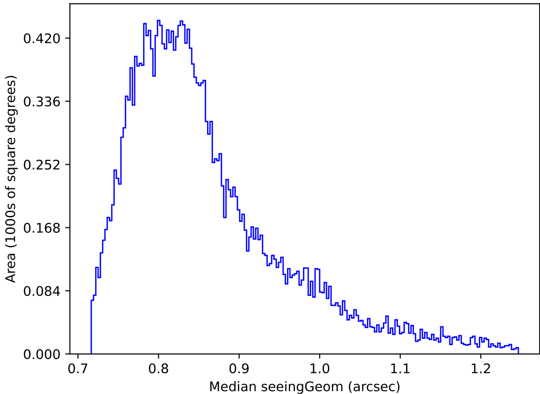
weather_cloudso30v3.4_10yrs Yr 1 all bands: Median seeingGeom
