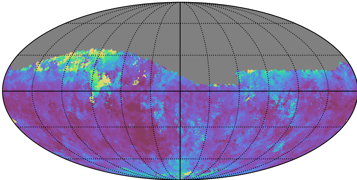
weather_cloudso30v3.4_10yrs Yr 1 z band: Median seeingEff
