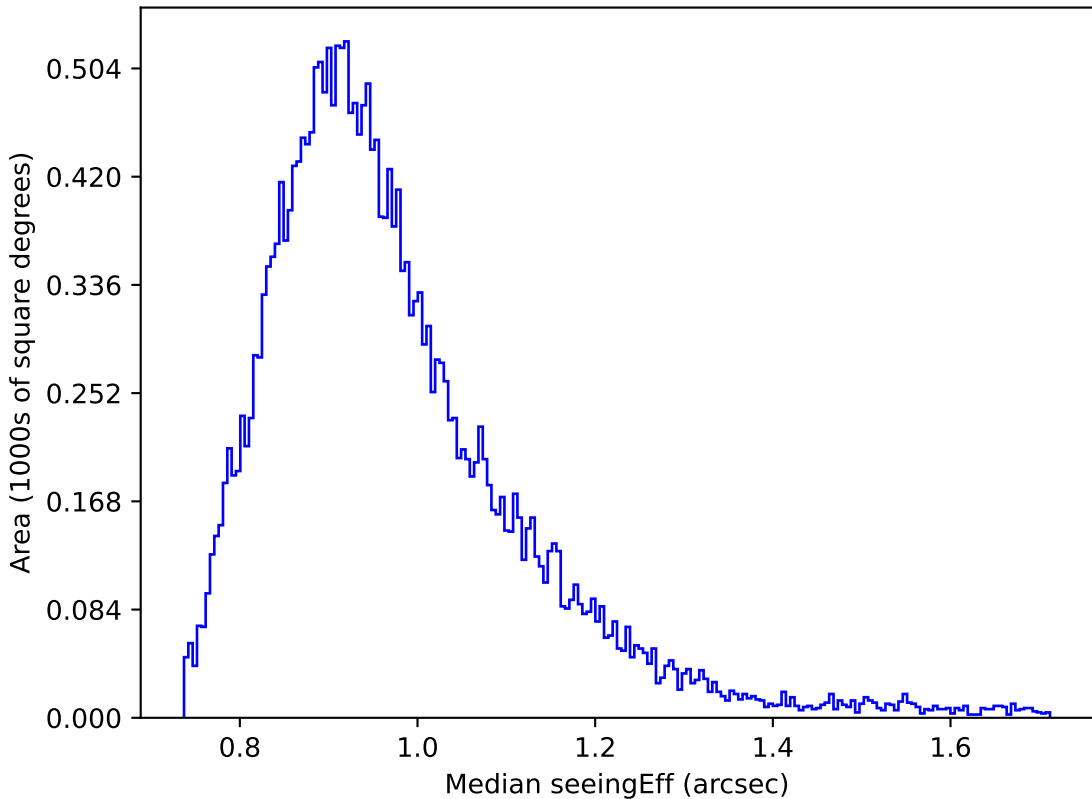
weather_cloudso30v3.4_10yrs Yr 1 z band: Median seeingEff
