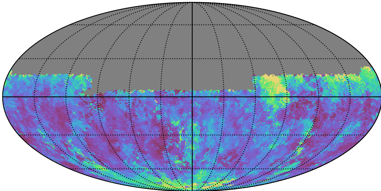
weather_cloudso30v3.4_10yrs Yr 1 y band: Median seeingEff
