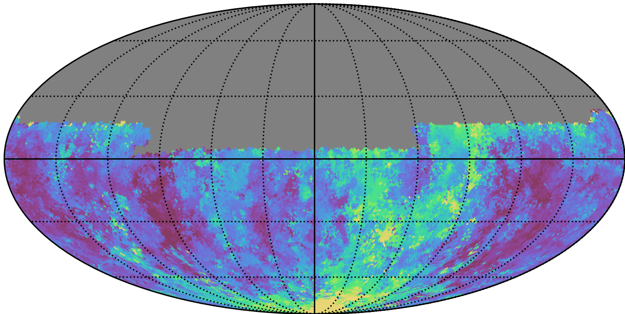
weather_cloudso30v3.4_10yrs Yr 1 u band: Median seeingEff
