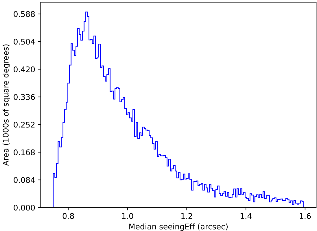
weather_cloudso30v3.4_10yrs Yr 1 r band: Median seeingEff
