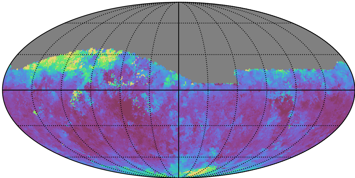
weather_cloudso30v3.4_10yrs Yr 1 i band: Median seeingEff
