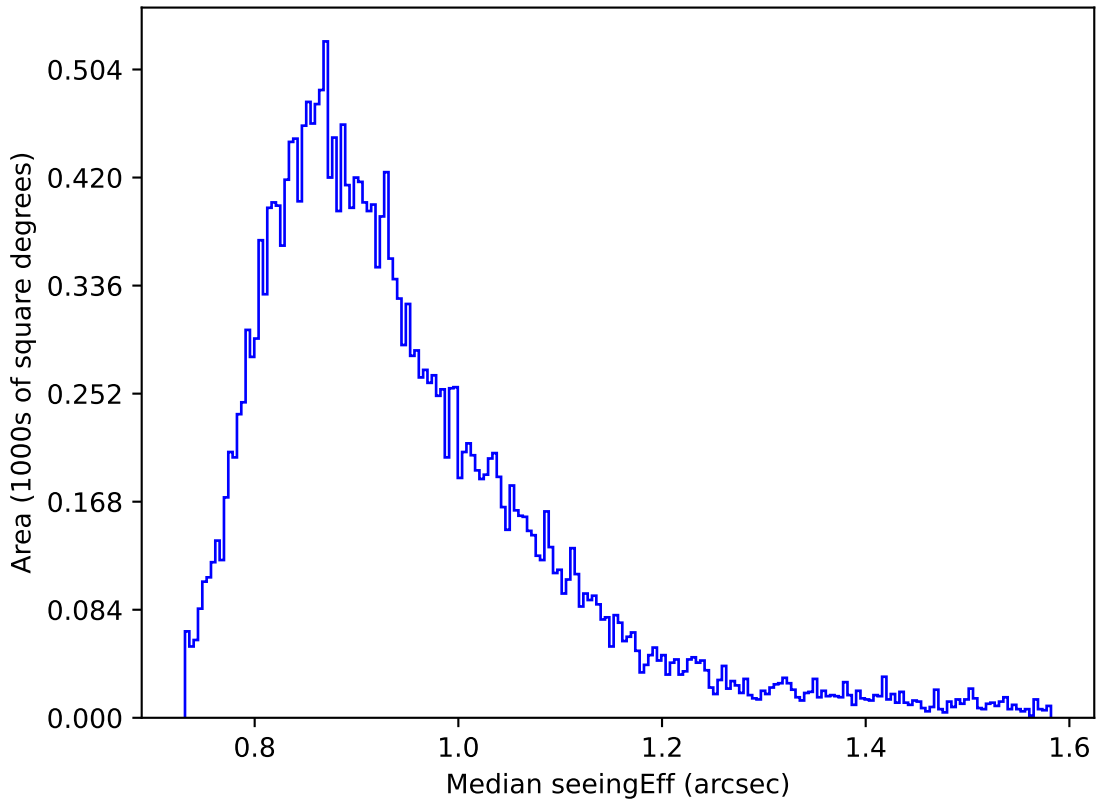
weather_cloudso30v3.4_10yrs Yr 1 i band: Median seeingEff
