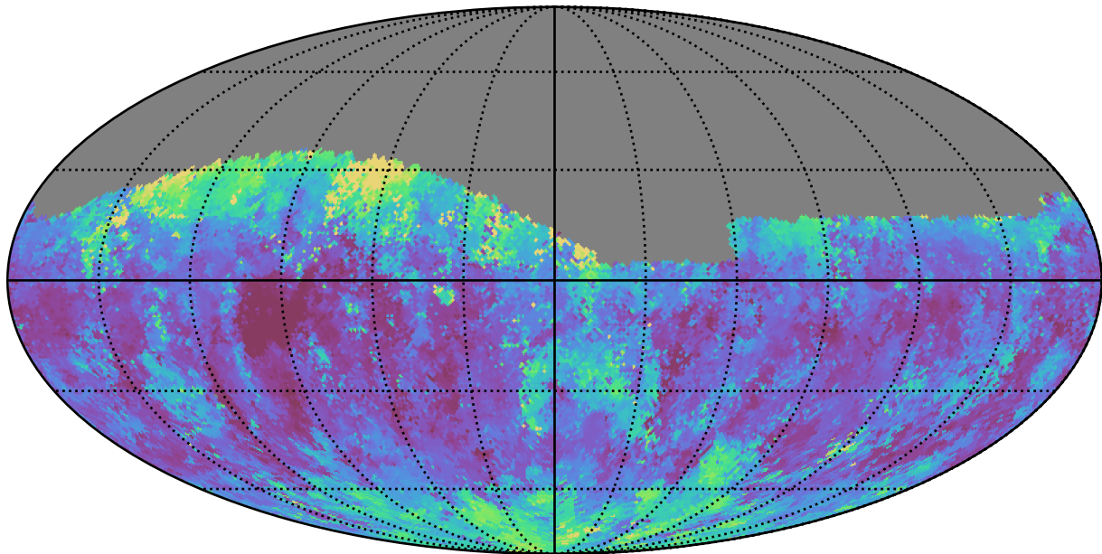
weather_cloudso30v3.4_10yrs Yr 1 g band: Median seeingEff
