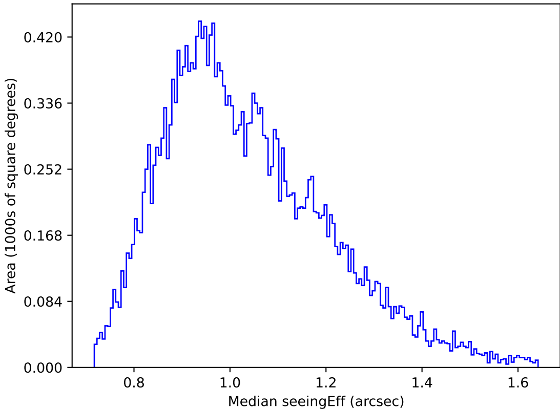
weather_cloudso30v3.4_10yrs Yr 1 g band: Median seeingEff
