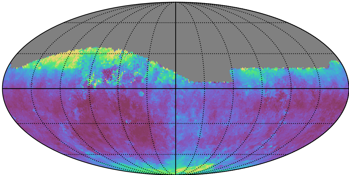
weather_cloudso30v3.4_10yrs Yr 1 all bands: Median seeingEff
